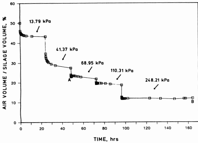
Figure 3. Air volume percentage vs. time for whole-plant corn silage test CMMC3.
