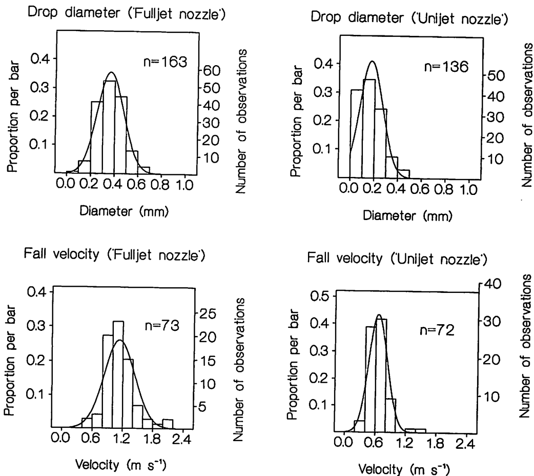
Fig. 2. Drop size distributions and drop fall-velocity distributions under Unijet and Fulljet nozzles (n represents the total number of observations).
