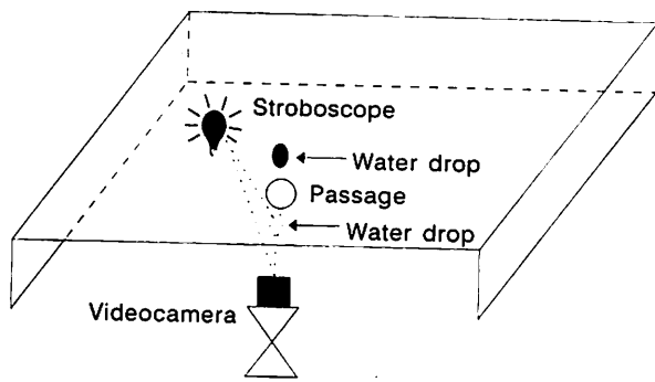
Fig. 1. Sketch of the experimental set-up for recording falling water drops onto a videotape.
