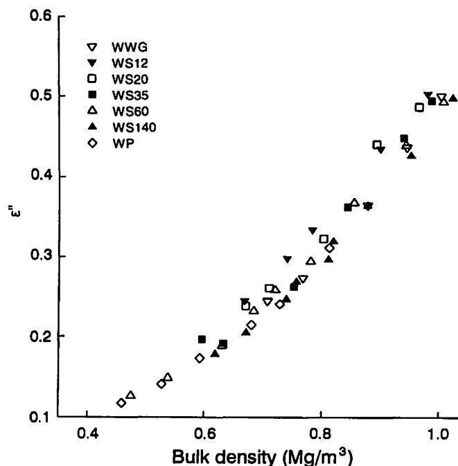
Fig. 13. Dielectric loss factor of various size fractions of wheat as a function of bulk density.
