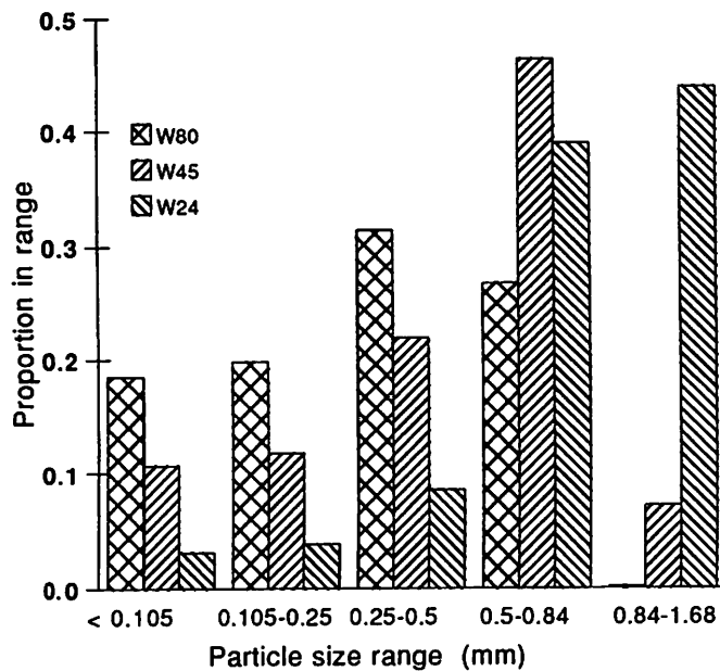
Fig. 9. Particle-size range (mm) and proportion of three ground wheat samples (W24, W45, W80).
