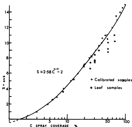
Figure 1. Calibration curve for zinc sprayed leaves standardized to Rd = 47.3 a = 19.1, b = 7.6 on Hunter Colour and Colour Difference Meter.
