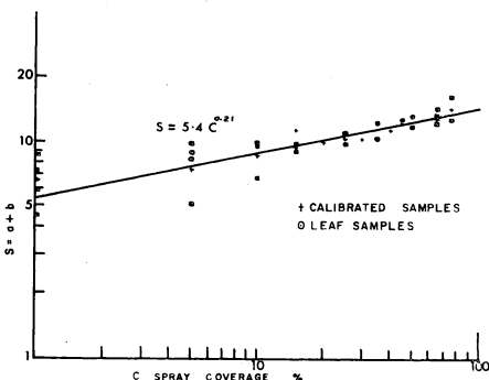
Figure 2. Calibration curve for copper sprayed leaves standardized to Munsell colour 5 BG 8/2 on Hunter Colour and Colour Difference Meter.
