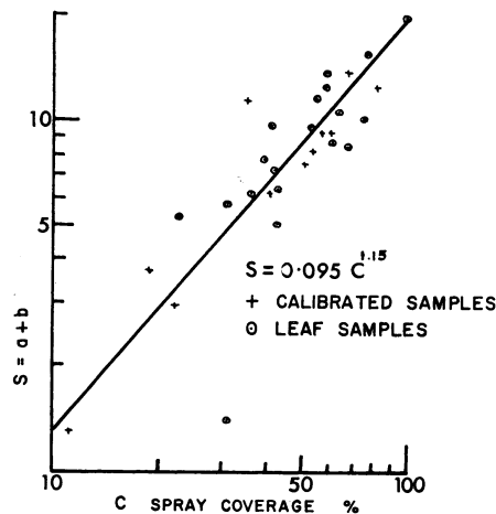
Figure 3. Calibration curve for copper sprayed leaves standardized to Munsell colour 2.5 YR 5/4 on Hunter Colour and Colour Difference Meter.
