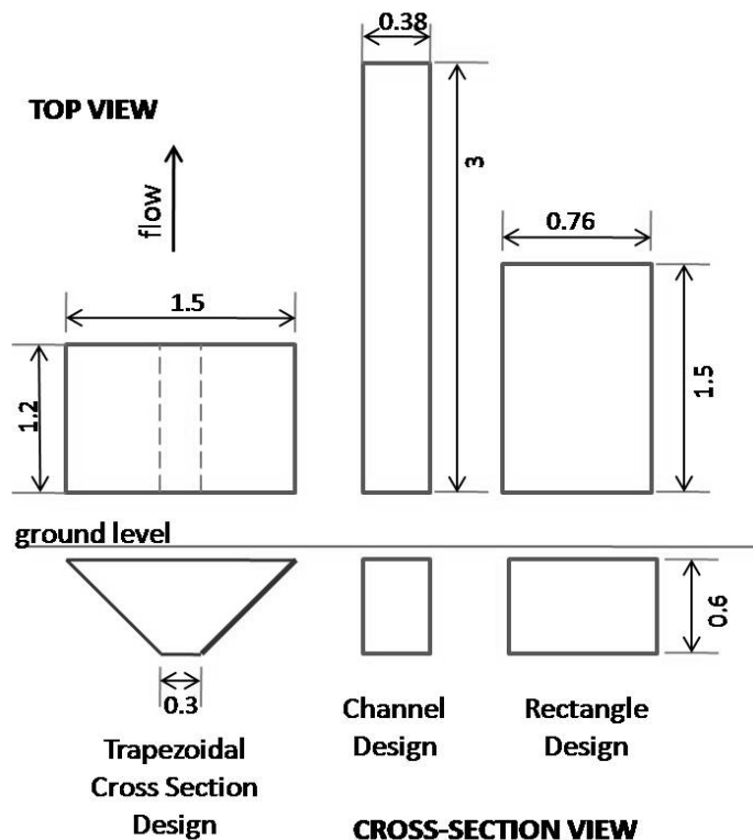
Figure 1. Schematic of three pilot bioreactors (all dimensions are in meters).
