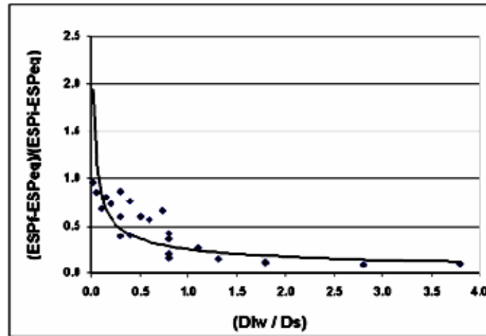
Figure 2: Soil desodification curve in the study area
