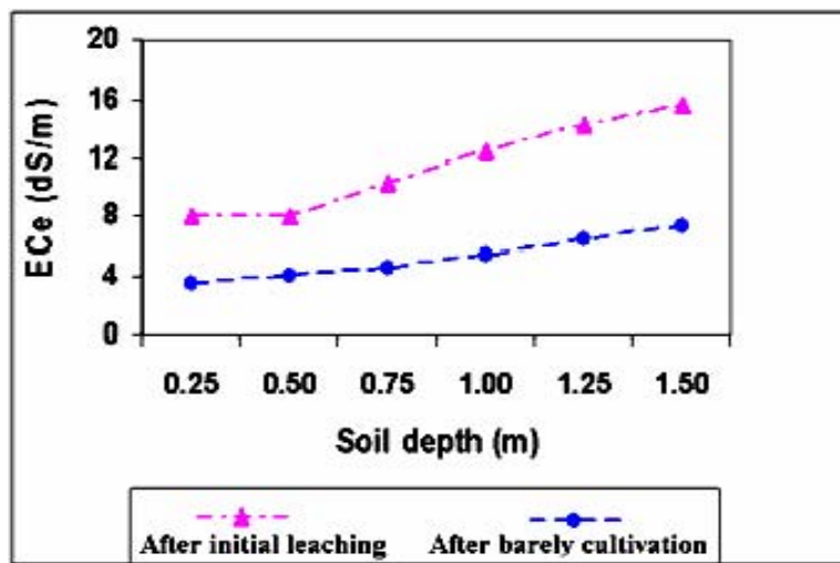
Figure 4: Salinity changes in the soil profile after barely cultivation
