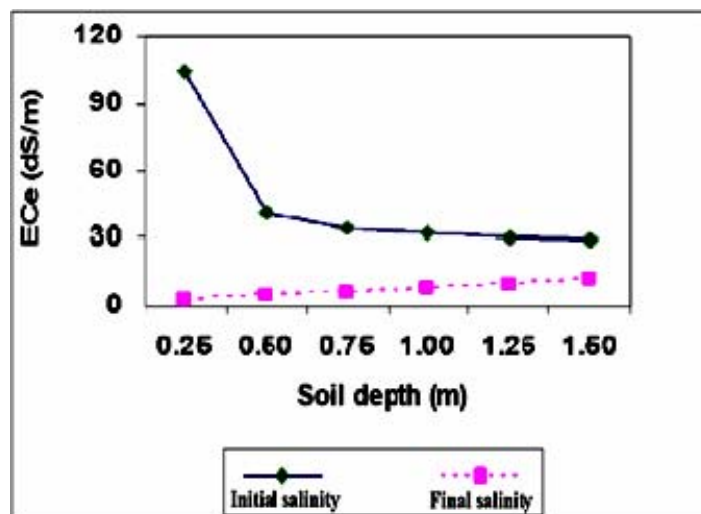
Figure 5: Salinity changes in the soil profile after initial leaching
