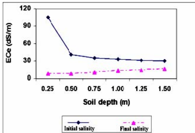
Figure 3: Salinity changes in the soil profile after initial leaching
