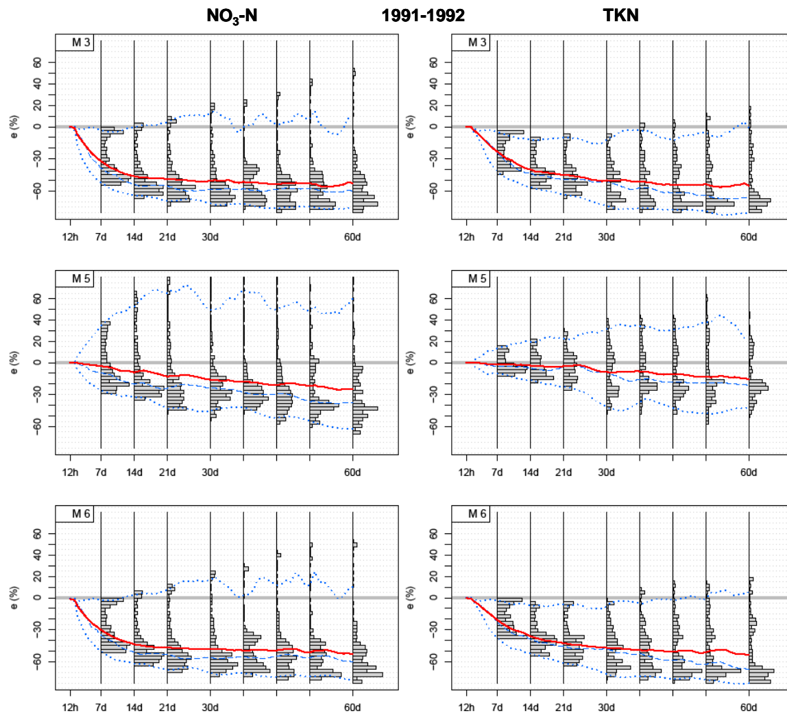
Figure 2. Bias and precision of annual N load estimates for 1991-92 by three different load estimate methods.
