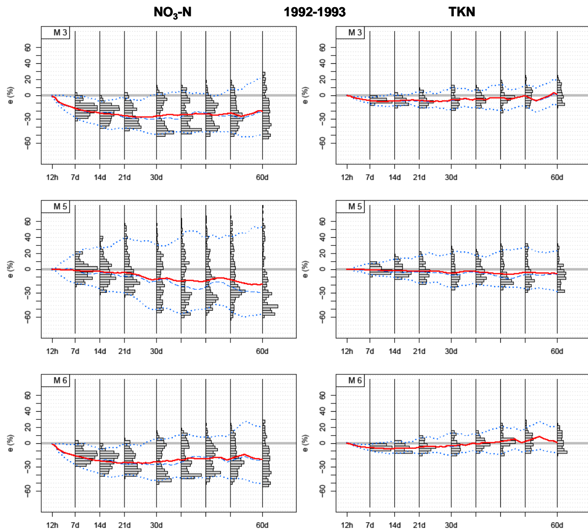
Figure 3. Bias and precision of annual N load estimates for 1992-93 by three different load estimate methods.
