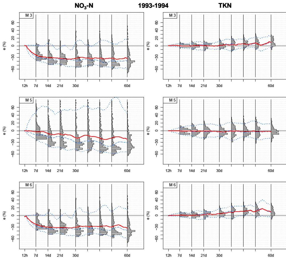
Figure 4. Bias and precision of annual N load estimates for 1993-94 by three different load estimate methods.
