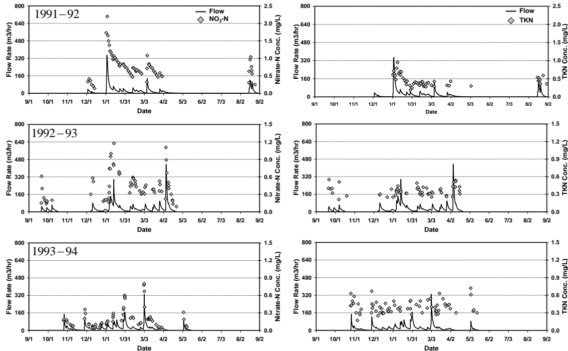
Figure 1. Measured flow and N concentrations for three years at the Carteret D1 site.
