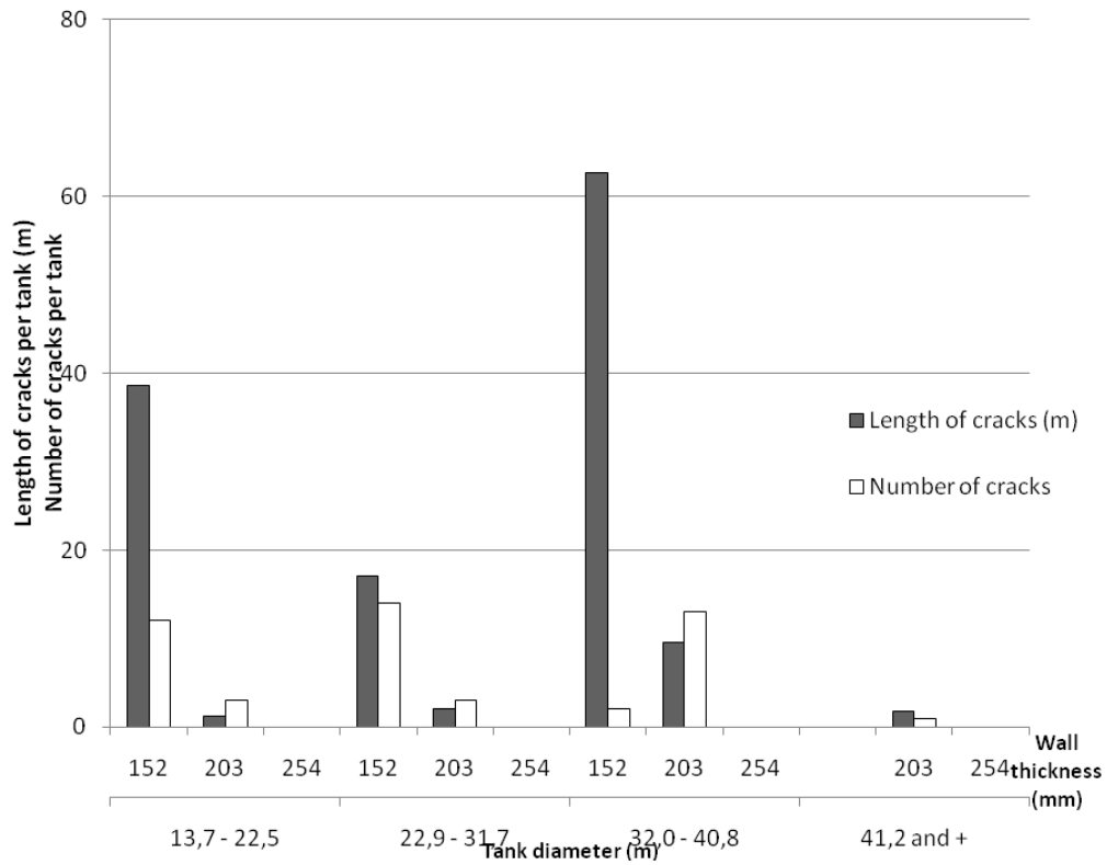
Figure 1. Crack length and number (per tank)
