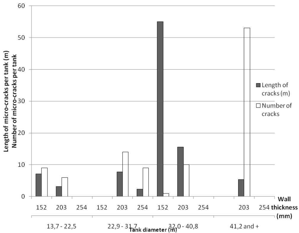
Figure 2. Micro-crack length and number (per tank)
