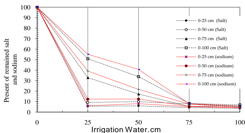
Fig.2 Comparison of applied irrigation water in washing salt and sodium in pilot No1
