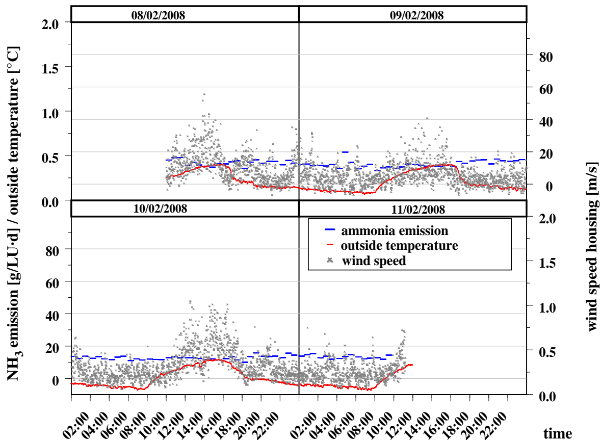
Figure 2: Diurnal \text{NH}_3 emission patterns [g/LU·d], wind speed in housing 3 m high [m/s] and outside temperature of the winter measurement.
